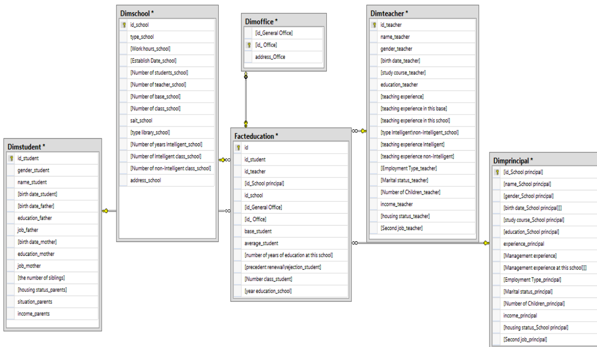
Figure 1. Scheme of Data Warehouse [7].
